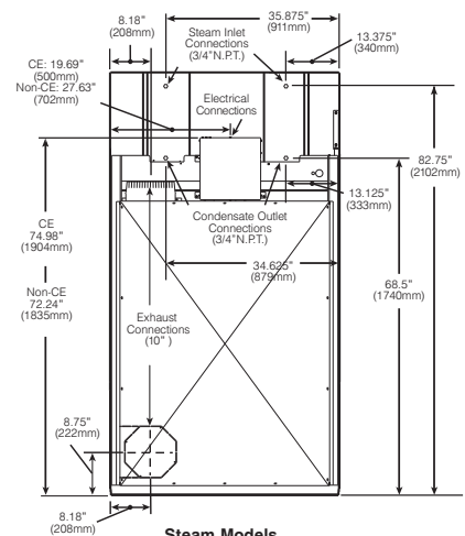
Steam Models
